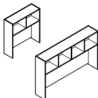
45" High Single Open Hutch 36 - 96 Widths 42 and 72 Widths Shown
